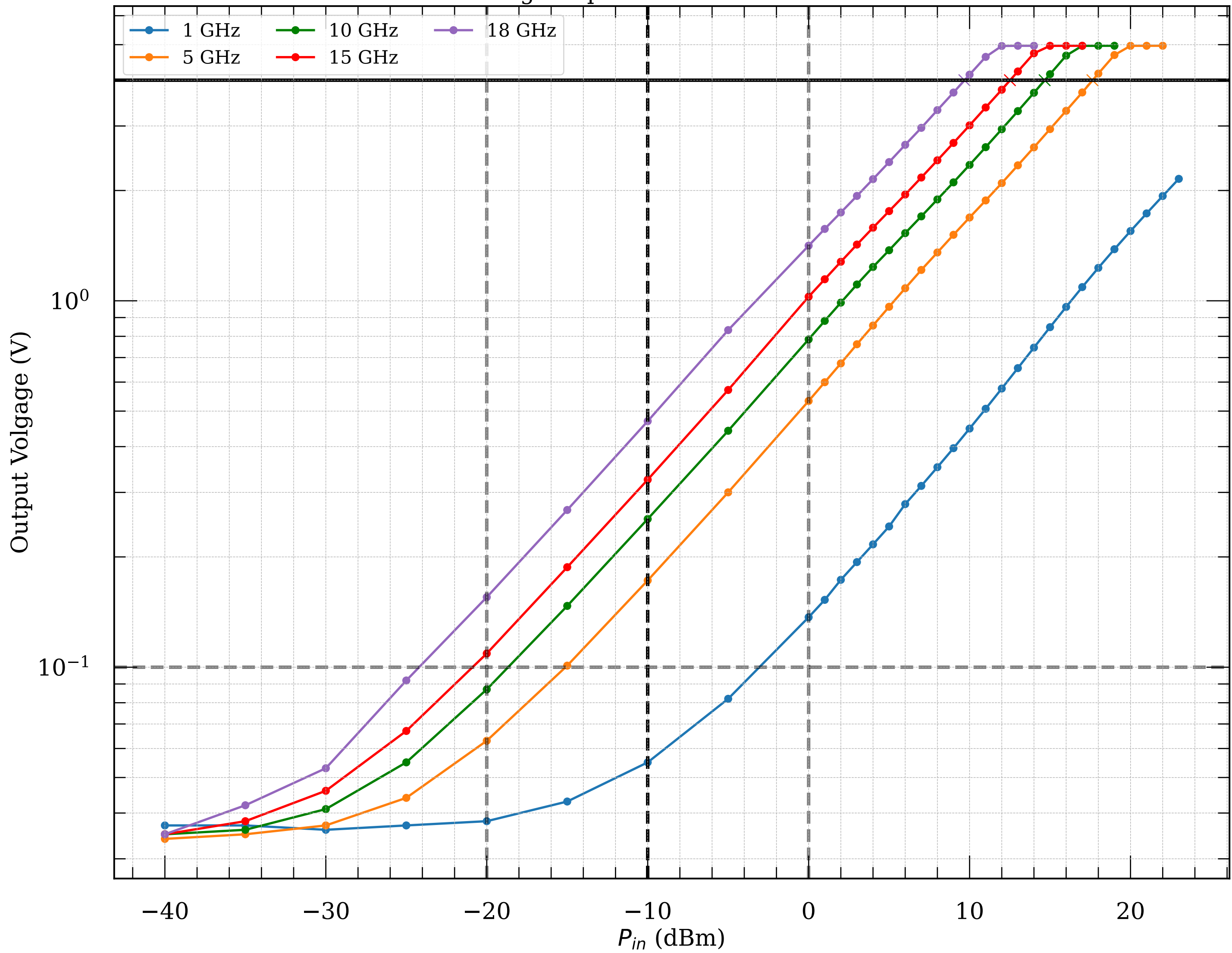
Measured voltage-to-power curve of detector module053
